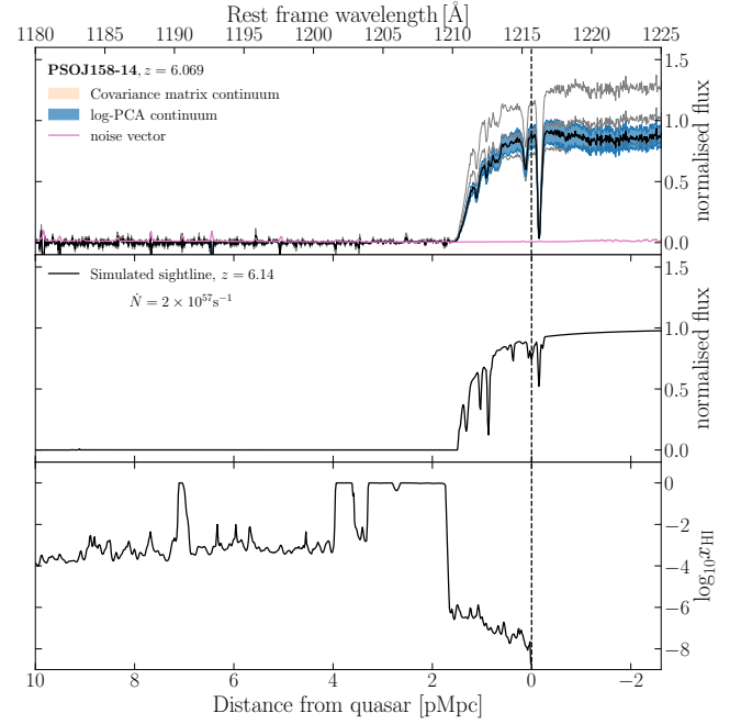
Figure 8. Top panel: Continuum-normalised spectrum of PSOJ158-14, for two continuum reconstruction methods, the log-PCA method (Chen et al. 2022) and the covariance matrix method (Greig et al. 2017a), shown in blue and orange, respectively. Shaded regions show the 1\sigma spread around the median value. (We use the log-PCA method for all quasars in this work.) Middle panel: A simulated spectrum showing an IGM damping wing at z = 6.14 for a quasar with magnitude -27 and age 1 Myr. Bottom panel: The ionised hydrogen fraction along the same simulated sightline. This reveals the neutral hydrogen regions that create the damping wing seen in the middle panel. At redshift 6.14, only one of 500 sightlines in our simulation shows this feature.
