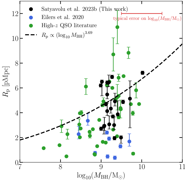
Figure 6. Proximity zone sizes as a function of supermassive black hole mass. Previous measurements for which black hole masses were available are shown in green and the targeted sample from Eilers et al. (2020) is shown in blue. Our measurements are shown in black. Our black hole masses are from Mazzucchelli et al. (in preparation). The typical error on the black hole masses is represented by the errorbar at the top right in red. All black hole masses are based on Mg II linewidths. The black dotted line shows the best fit curve to our measurements and previous measurements excluding Eilers et al. (2020). For obtaining the best fit, a relatively homogeneous subset of quasars with -26.8 < M_{1450} < -27.2 and 6.0 < z < 6.2 was used. A power-law relationship was assumed between the quasar proximity zone size and logarithm of the black hole mass, as motivated in the text.
